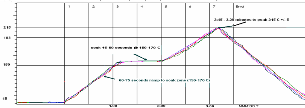
Ramp-Soak-Spike (RSS): Recommended profile.
